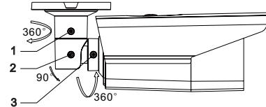
Figure 2-7 3-axis Adjustment
