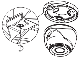
Figure 2-3 Install the Turret Camera
