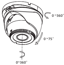
Figure 2-4 3-axis Adjustment
